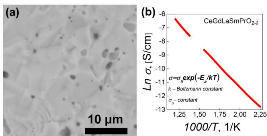
Figure 3. Typical microstructure of the fracture surface of bulk samples for example of \text{CeGdLaSmPrO}_{2-\delta} (a) and temperature dependence of the electrical conductivity in \ln\sigma ( 1/T ) coordinates (b)
