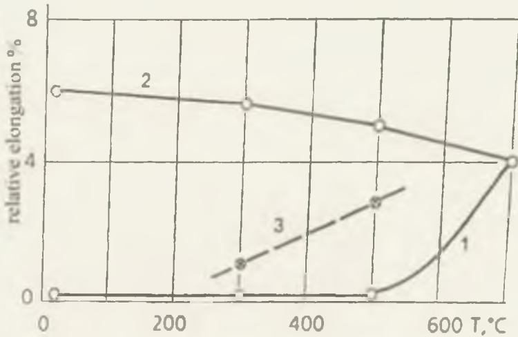
Figure 6. The temperature dependence of relative extension of a low alloyed chromium irradiated with a fluence of approximately 0.1 displacements per atom (dpa) (1), the initial material (2), and the material irradiated and deformed by bends (3).
