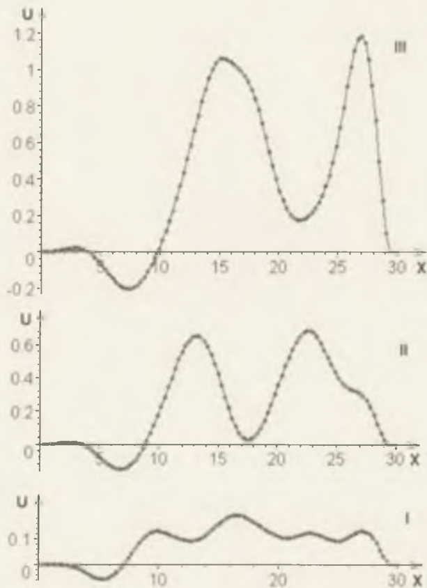
Figure 3. The plots of the Eq. (10) solution constructed for the time interval \Delta t = 7.3 . The plot I corresponds to u(x, 0) = 0.2 ; the plots II and III do u(x, 0) = 0.5 и u(x, 0) = 1 , respectively.
