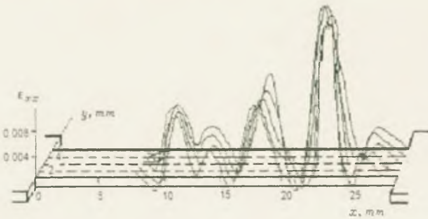
Figure 4. The pattern of the deformation distribution along a sample during the initial straining stages (Figure 1 of the work [11]).
