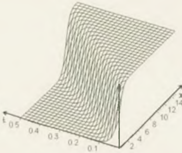
Figure 2. Three-dimensional plot of step propagation of plastic deformation in sliding plane.
