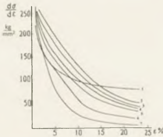
Figure 7. The dependence of deformation hardening coefficient on relative plastic deformation \epsilon : The curve 1 corresponds to unirradiated nickel; the curves 2, 3, 4, 5, 6, and 7 correspond to nickel irradiated by electrons with energy of 225 MeV (dose of radiation is 10^3, 10^2, 10^1, 2 \times 10^1, 5 \times 10^1 , and 5 \times 10^0 (dpa), respectively).
