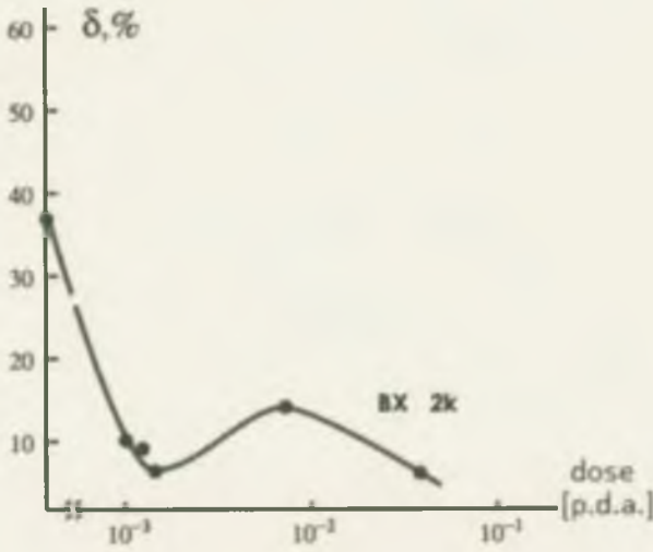
Figure 10. The experimental dose dependence of elongation of low-activated alloy based on chromium VCh-2 K under (e, \gamma )—Beam radiation.
