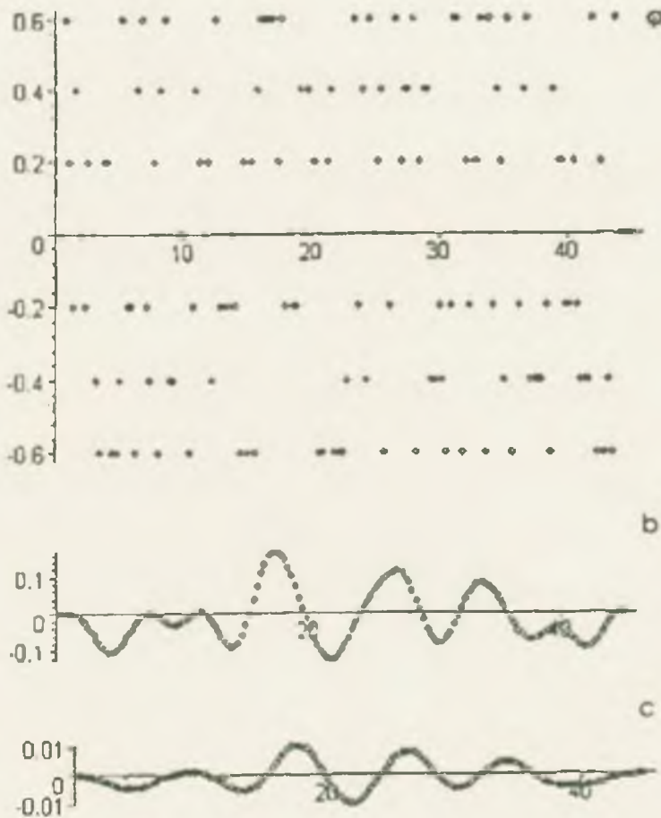
Figure 5. The spatially temporary evolution of the dislocation density, according to Eq. (10) with the right side being equal to 10^{-3} in relative units. The account time is 0.3 (a), 1 (b), and 5 s (c).
