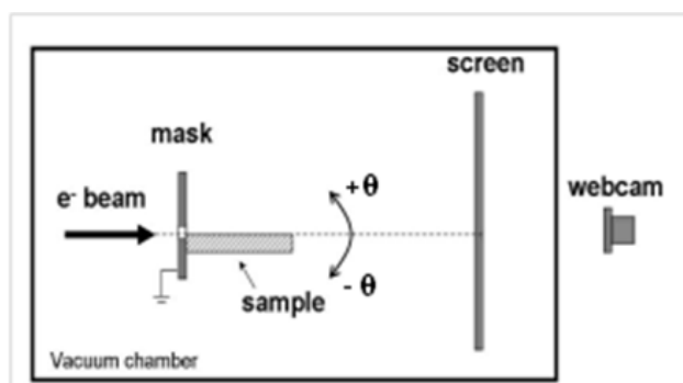
Figure 1. The diagram of experimental setup in vacuum chamber ( \theta – tilting angle).
